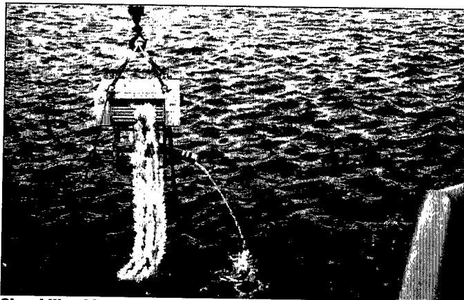
Oleophilic skimmer.
