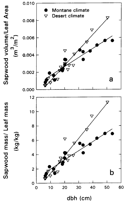
FIG. 2. Whole-tree relationships between sapwood and leaves for Pinus ponderosa in montane and desert climates. (a) Whole-tree sapwood volume : leaf area ratios (SLR) vs. dbh for Pinus ponderosa in montane and desert climates. For montane trees, SLR = -0.00057 + 0.00010(\text{dbh}) , r^2 = 0.90 . For desert trees, SLR = -0.00077 + 0.00018(\text{dbh}) , r^2 = 0.92 . Slopes differed significantly, ANCOVA, P < 0.001 . (b) Whole-tree sapwood mass : leaf mass ratios (SLM) vs. dbh for Pinus ponderosa in montane and desert climates. For montane trees, SLM = 0.701 + 0.127(\text{dbh}) , r^2 = 0.90 . For desert trees, SLM = -1.030 + 0.243(\text{dbh}) , r^2 = 0.92 . Slopes differed significantly, ANCOVA, P < 0.001 .
