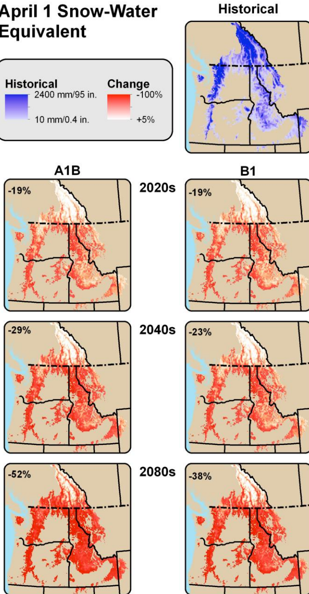
Figure 20. SWE projected decline over time.
