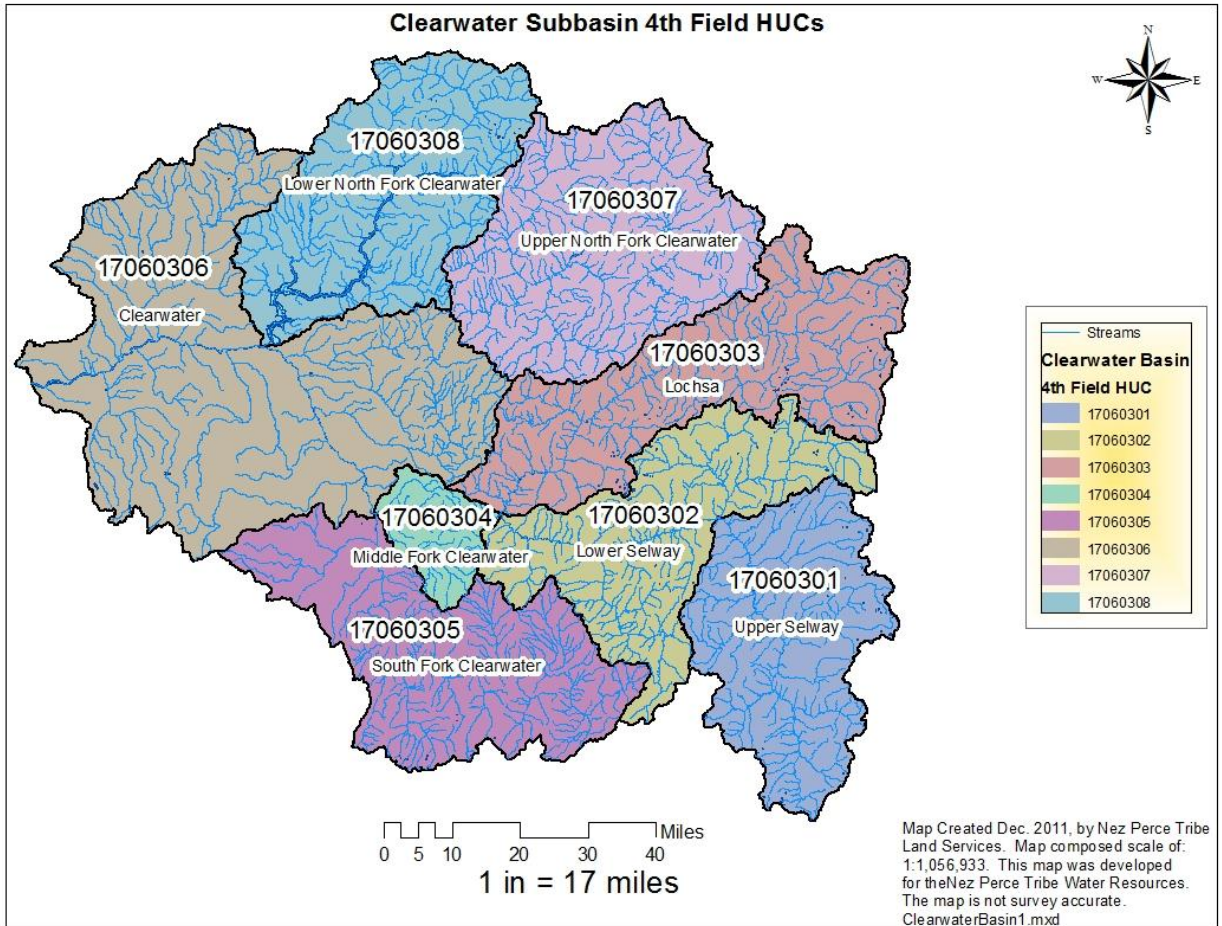
Figure 16. Clearwater River Subbasin 4th Code Hydrologic Unit Codes (HUCs).
