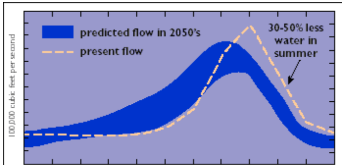
Figure 21. Naturalized Columbia River streamflow at The Dalles currently and in 2050. The blue band indicates the upper and lower bounds of projected average streamflow in the 2050s (CIG 2011).
