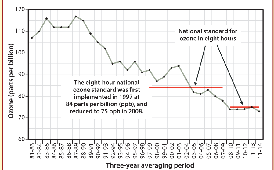
Figure 11. Maine annual statewide maximum eight-hour design value for ozone over time with the National Ambient Air Quality Standard (NAAQS) noted as red lines. The NAAQS standard was reduced from 84 parts per billion (ppb) to 75 ppb in 2008. The design value for each monitoring site is the average of the fourth highest maximum daily eight-hour ozone concentration for each of three consecutive years as long as data recovery rates meet requirements. Data and further details available at maine.gov/dep/air/ozone/aqtrends.html .
