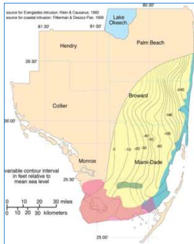
Figure 43 - Biscayne Aquifer lower contour in feet relative to mean sea level. Areas shown in blue and pink are the saltwater intrusion zones. (USGS)
