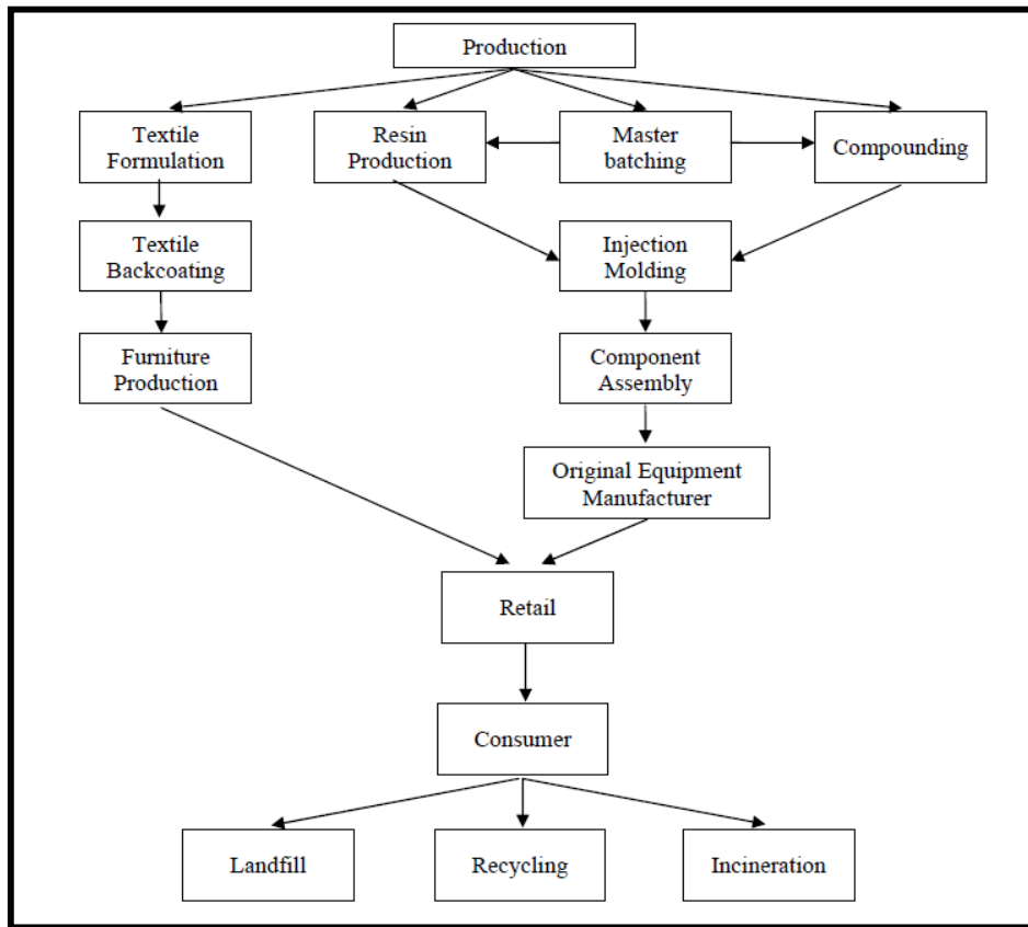
Figure 2-2. Idealized life cycle of polybrominated diphenyl ethers if all information is available to complete the analysis.
