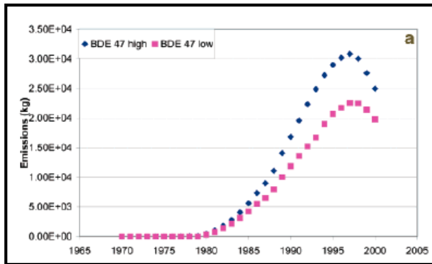
Figure 2-4. Volatilization of BDE 47 from PBDE-treated consumer products in the U.K.
