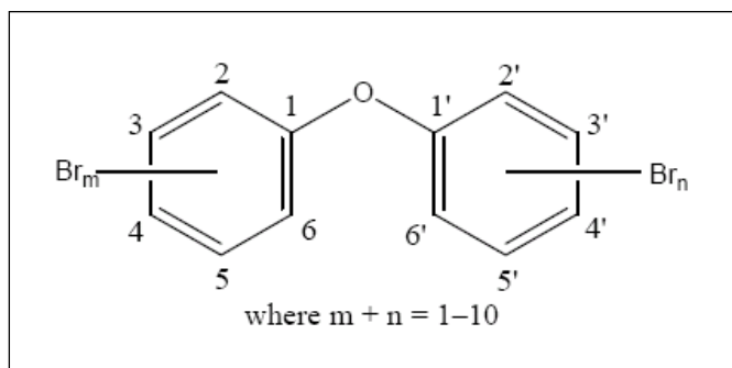
Figure 2-1. General structure of polybrominated diphenyl ethers.
