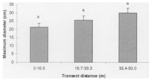
FIGURE 5. Effect of transect distance on maximum tree diameter, all species combined. Values are means and standard errors. No significant effect of distance (ANOVA; p > 0.05 ) was detected.
